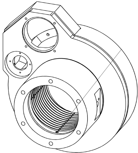
Housing for knife adjustment for Emulsifier 225 part number 308967
