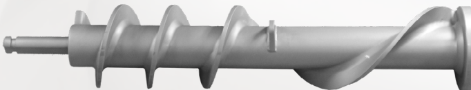
Worm AG 200 Grinder Wolfking®/CFS®/GEA® type
